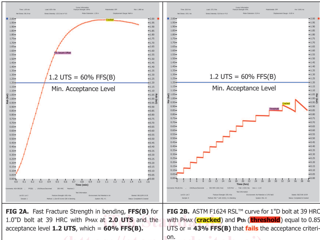
FIG. 2 Fast Fracture Testing and Step Loading Profile
