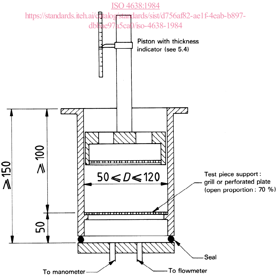
Figure 3 — Measurement cell (cylindrical section)
