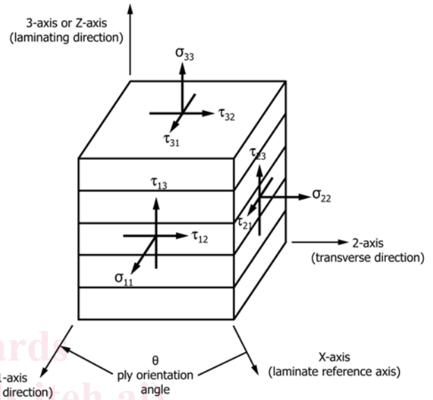
FIG. 1 Material Coordinate System
