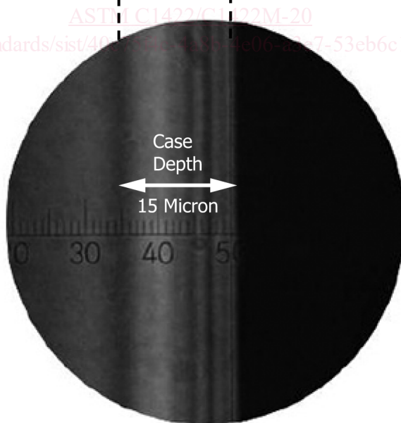
FIG. 2 (a)(b) Photo from Polarizing Microscope Using Monochromatic Filter and Eyepiece Reticle to Measure Case Depth
