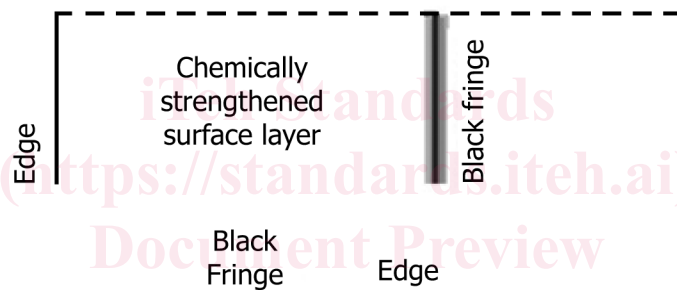
FIG. 2 (a) Case Depth and Birefringence Measurement Positions
