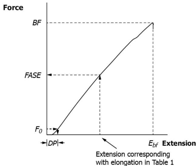
FIG. 1 Force-elongation Curve
