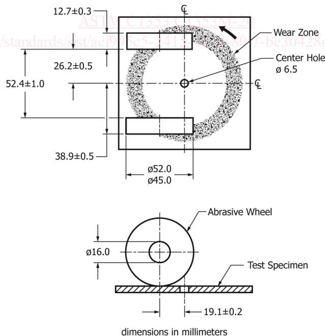
FIG. 2 Diagrammatic Arrangement of Rotary Platform Abraser Test Set-up
