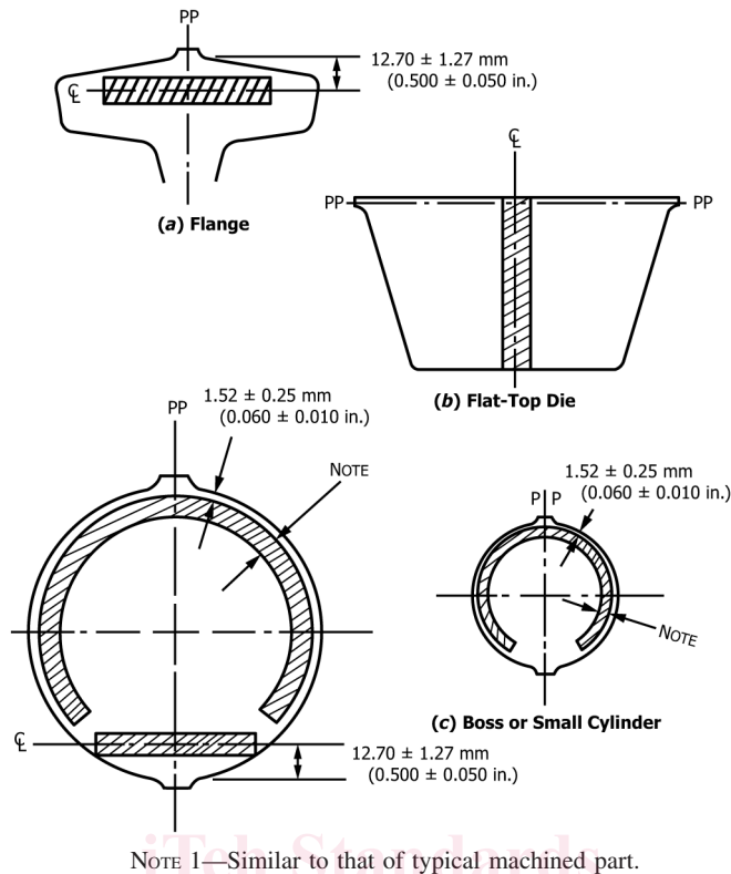
NOTE 1—Similar to that of typical machined part. FIG. 1 Recommended Specimen Type and Location for Various Configurations of Die Forgings
