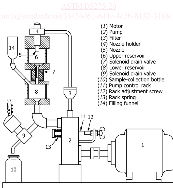
FIG. A1.1 Fuel Injector Shear Stability Test (FISST) (Schematic)
