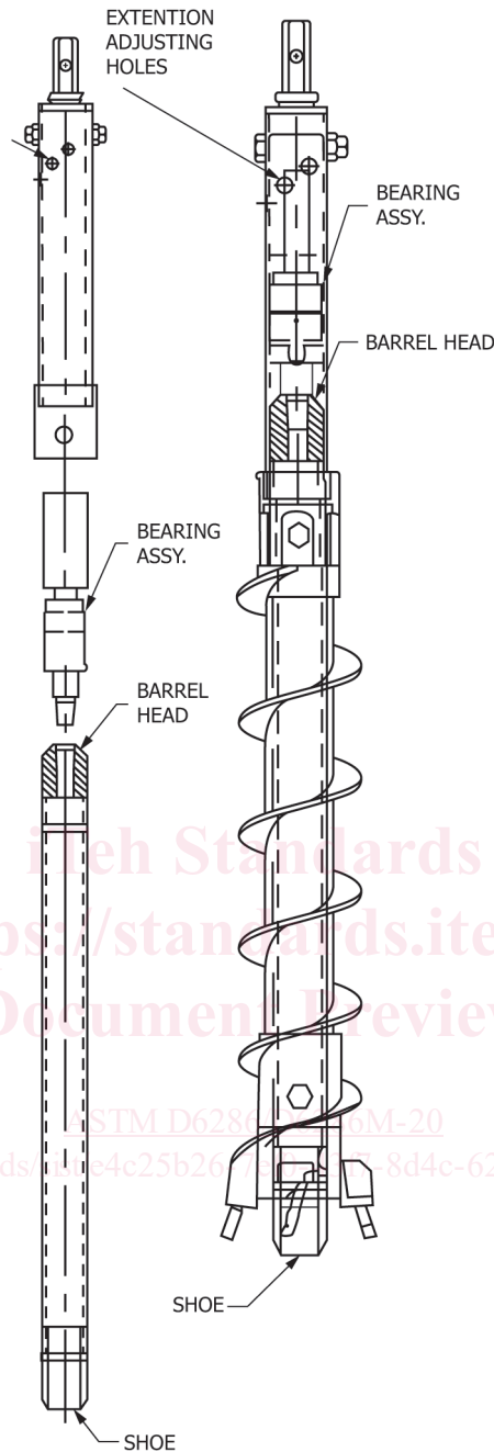
FIG. 2 Hollow-Stem Auger drilling system showing the continuous soil sample barrel (Diedrich Drill)
