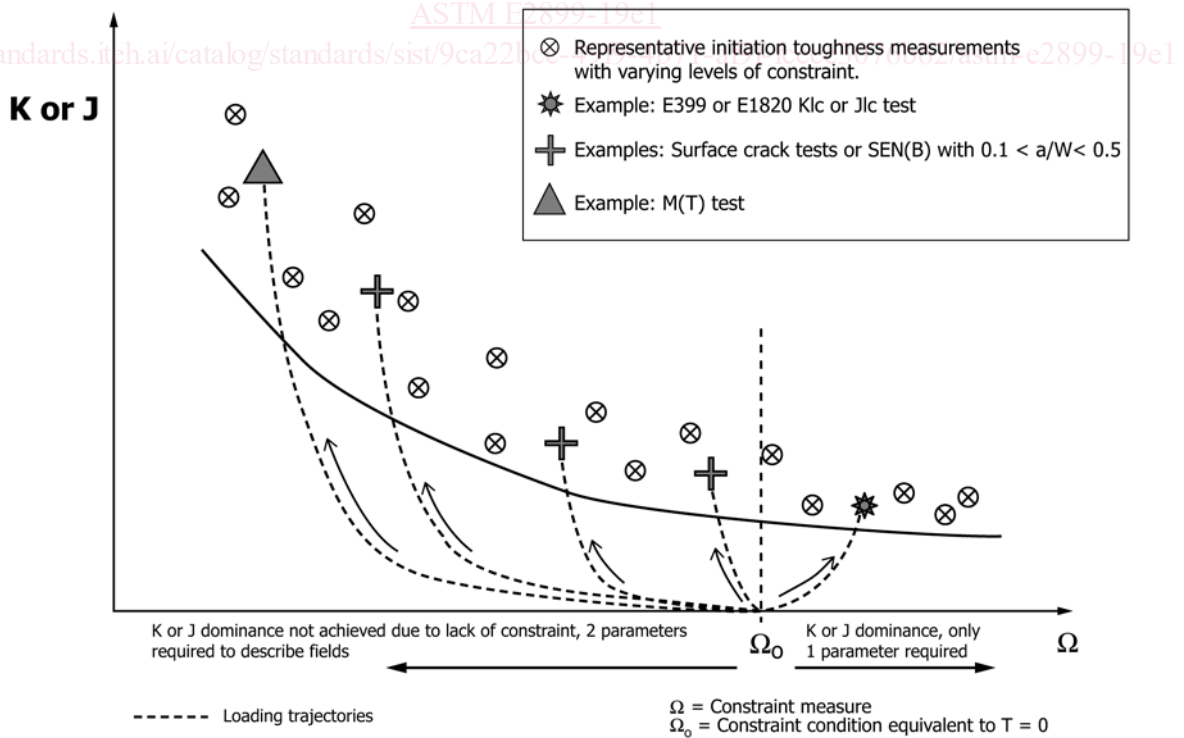
FIG. 2 Toughness-Constraint Locus with Example Trajectories
