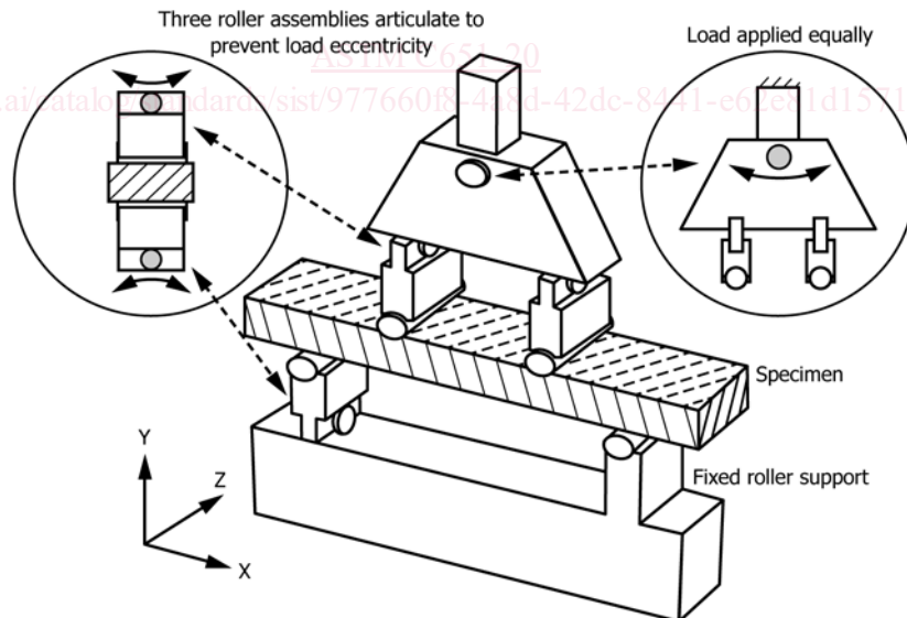
FIG. 1 Beam with Four-Point Loading
