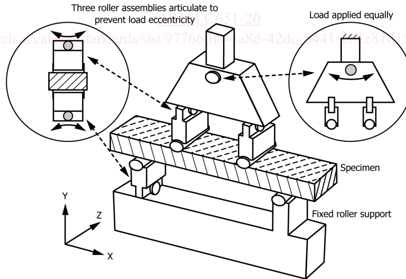
FIG. 1 Beam with Four-Point Loading
