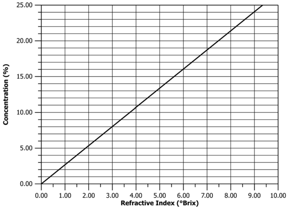
FIG. 8 Typical Refractive Index (Degrees Brix) Versus Quenchant Concentration Relationship
