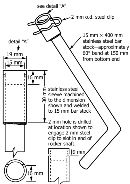
FIG. 2 Rocker Shaft Removal Tool
