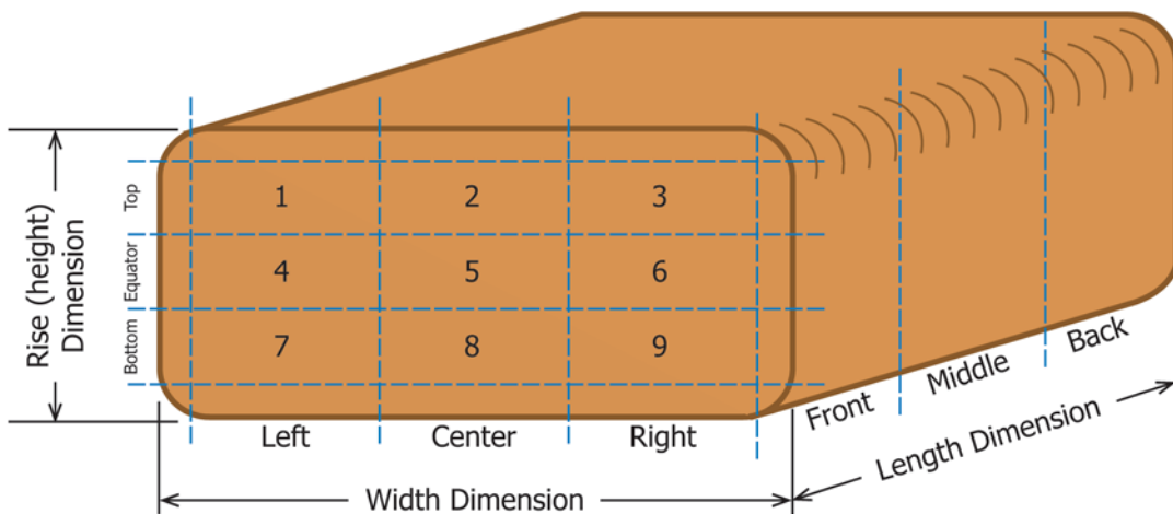
FIG. A1.2 Bun Position Definitions for Box-Pour PIR
