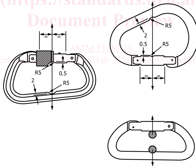
FIG. 2 Test-Fixture Minor Axis Test Pin Location
