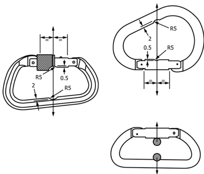
FIG. 2 Minor Axis Test Pin Location
