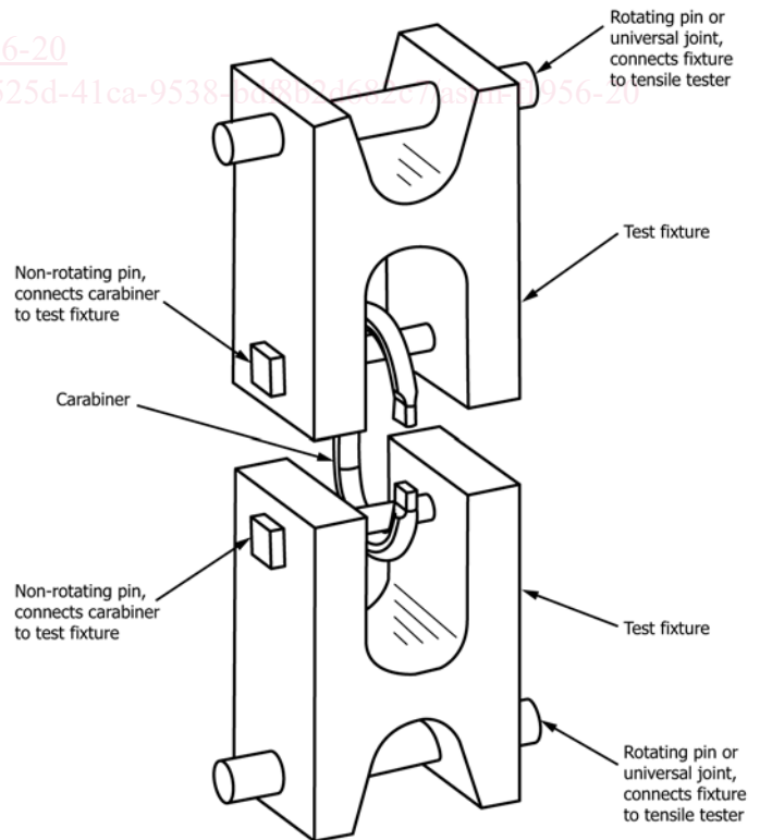
FIG. 1 Major Axis Test Setup
