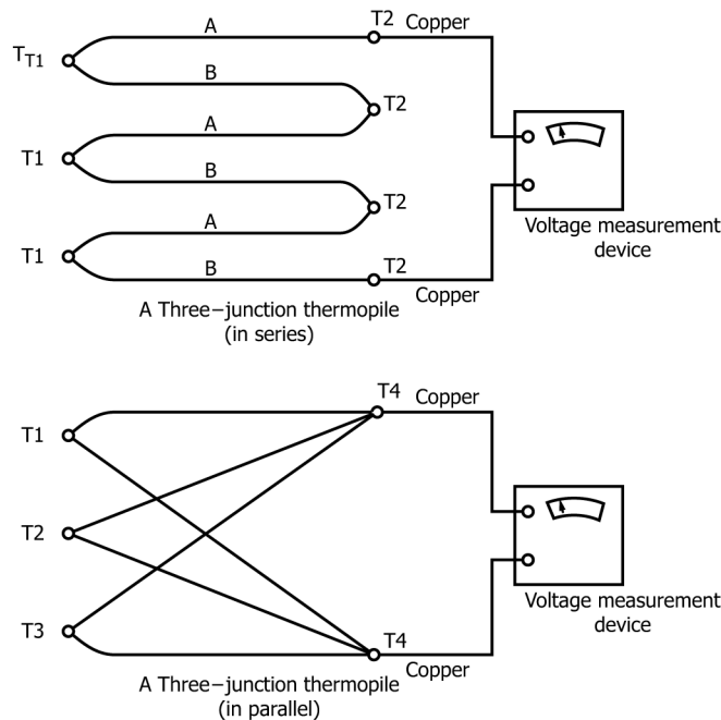
FIG. 6 Multiple-Junction Thermopiles
