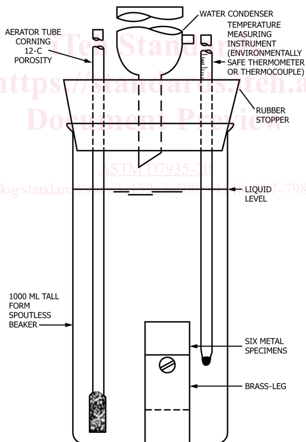
FIG. 1 Metal Specimens and Equipment for 336-h 336 h Corrosion Test
