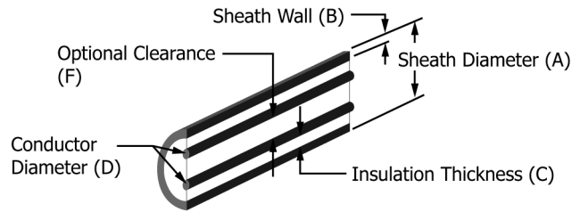
FIG. 2 Sheathed RTD Material Construction
