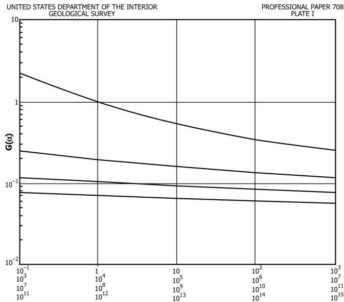
FIG. 2 Logarithmic Plot of \alpha Versus G(\alpha)
