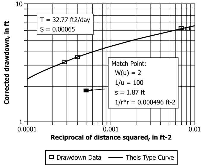
FIG. 5 Analysis of Drawdown Data Corrected for Partial Penetration Assuming an Anisotropy of 0.17, Estimated T of 35.42 \text{ft}^2 (3.29 \text{m}^2 )/day, and S of 0.00055 Yields a Revised T of 32.77 \text{ft}^2 (3.04 \text{m}^2 )/day and S of 0.00065
