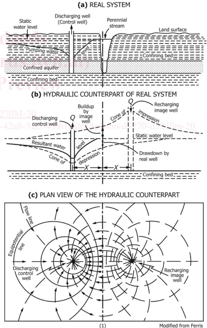
NOTE 1—Modified from Ferris and others (1) and Heath (2). 3 FIG. 1 Diagram Showing Constant-Head Boundary
