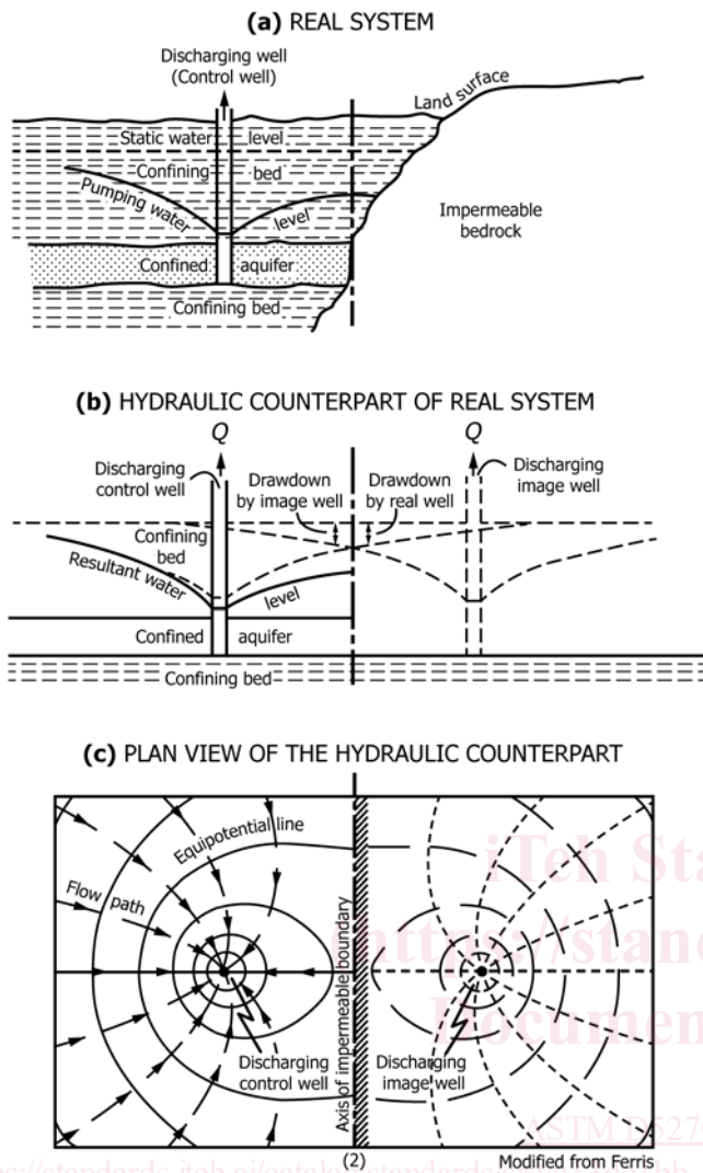
NOTE 1—Modified from Ferris and others (1) and Heath (2). FIG. 2 Diagram Showing Impermeable Boundary
