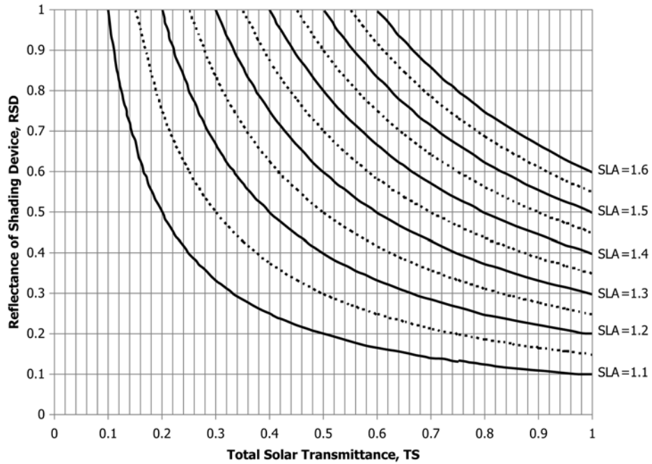
FIG. 3 Solar Load Adjustment Factor, SLA
