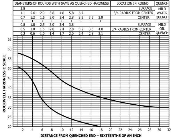
FIG. 3 Limits for Hardenability Band 1335 H
