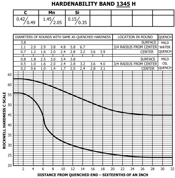
FIG. 5 Limits for Hardenability Band 1345 H
