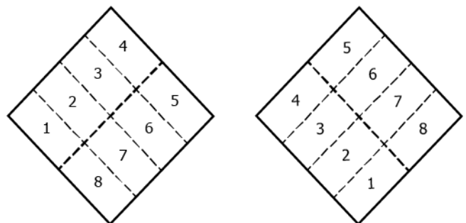
Rounds 1 and 3 Rounds 2 and 4 FIG. 1 Order of Tamping in Molding of Test Specimens
