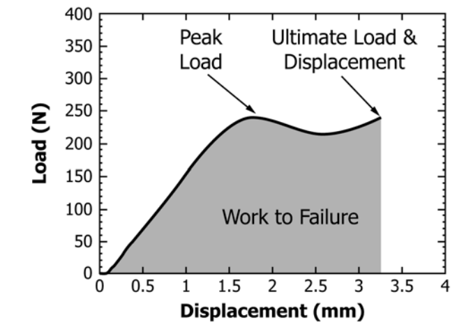
FIG. 2 Features of the small punch test load versus displacement curve for PEEK, including the peak load, ultimate load & displacement, and work to failure
