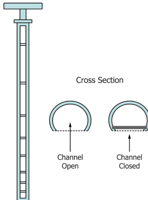
FIG. 1 Scoop-Slide Sampler
