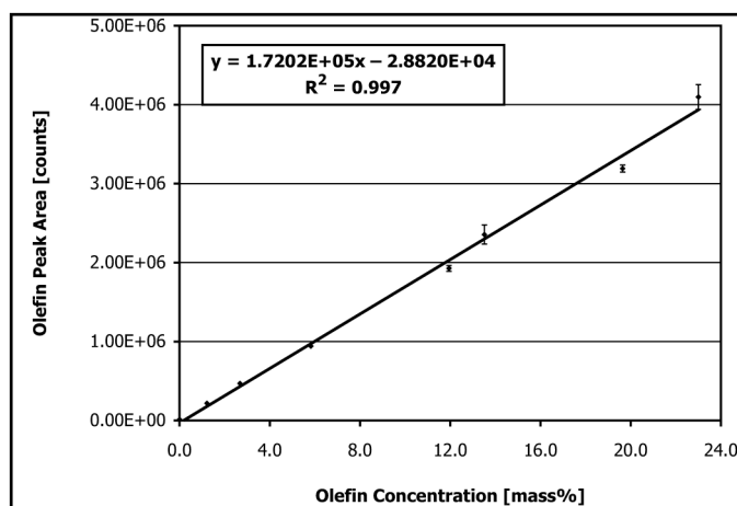
FIG. 4 Typical Calibration Curve
