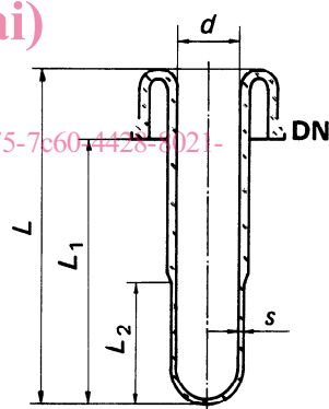
FIGURE 5 – Gaine thermométrique
