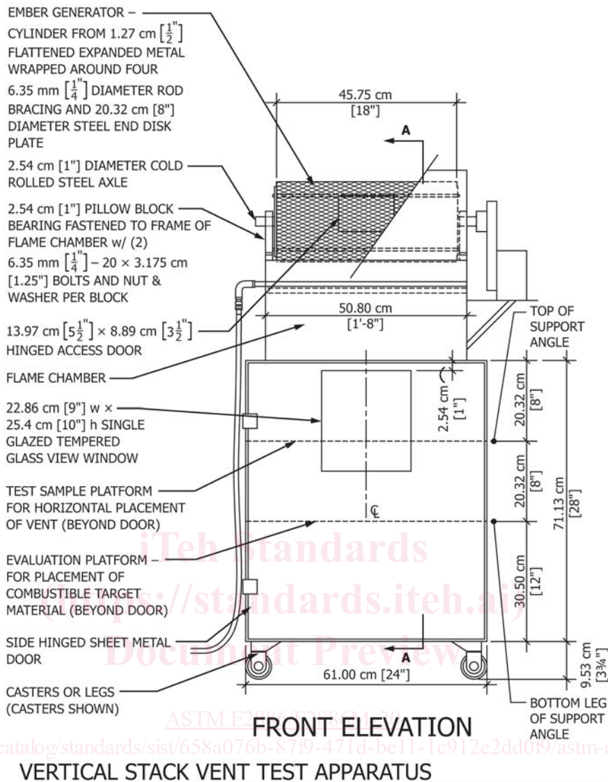
FIG. 1 Ember Apparatus, Front View
