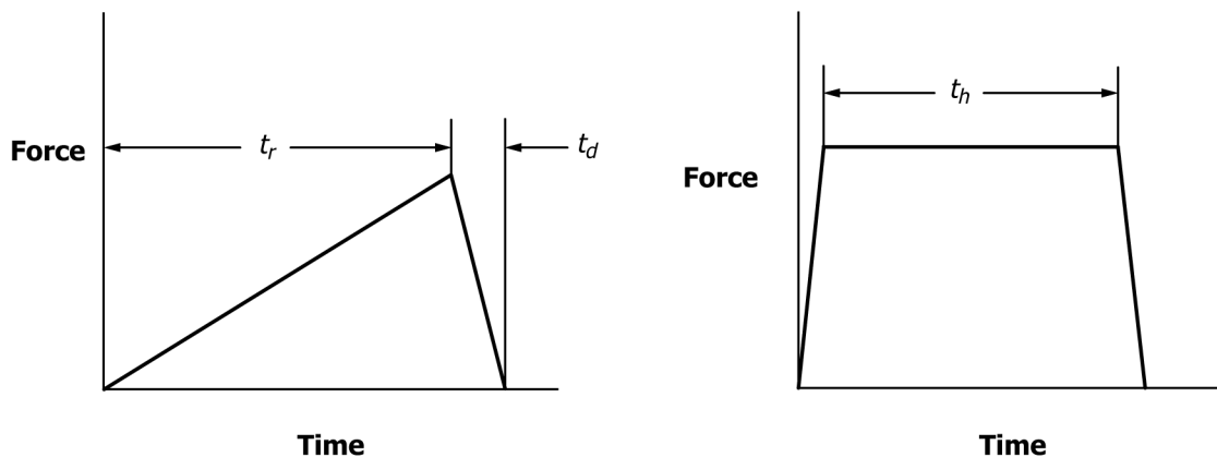
FIG. 2 Example Creep-Fatigue Cycle Shapes
