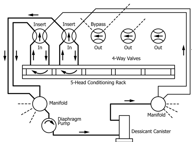
FIG. 2 Conditioning System
