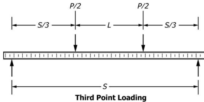
(c) 4-Point Loading (C393/C393M and D7249/D7249M Non-Standard Configuration)
