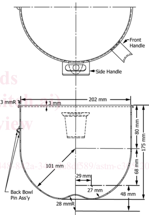
FIG. 3 Mixing Bowl
