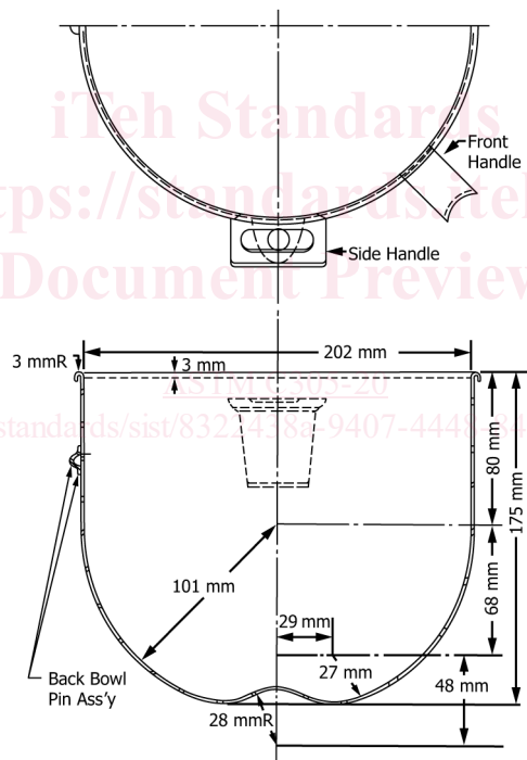
FIG. 3 Mixing Bowl
