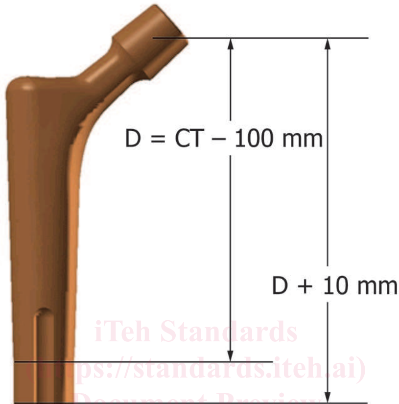
FIG. 4 Boundary Condition Location for Hip Stem Length of CT > 250 mm
