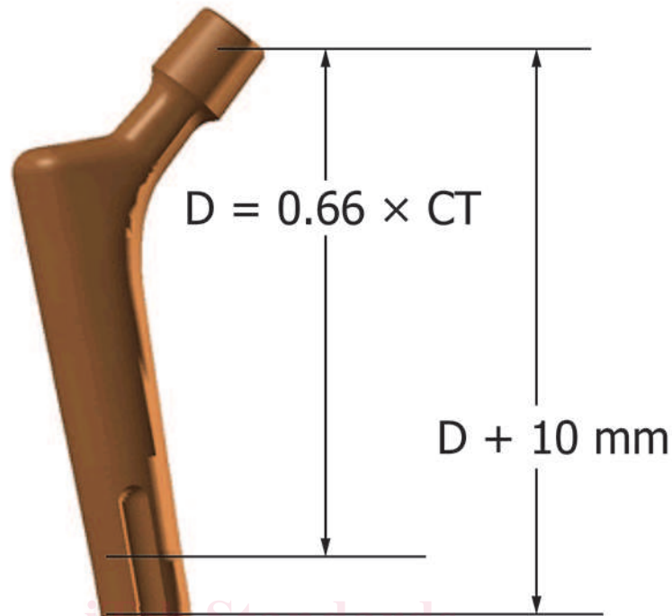
FIG. 2 Boundary Condition Location for Hip Stem Length \leq 120 mm
