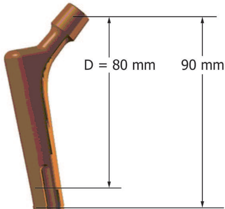
FIG. 3 Boundary Condition Location for Hip Stem Length of 120 mm < CT ≤ 250 mm
