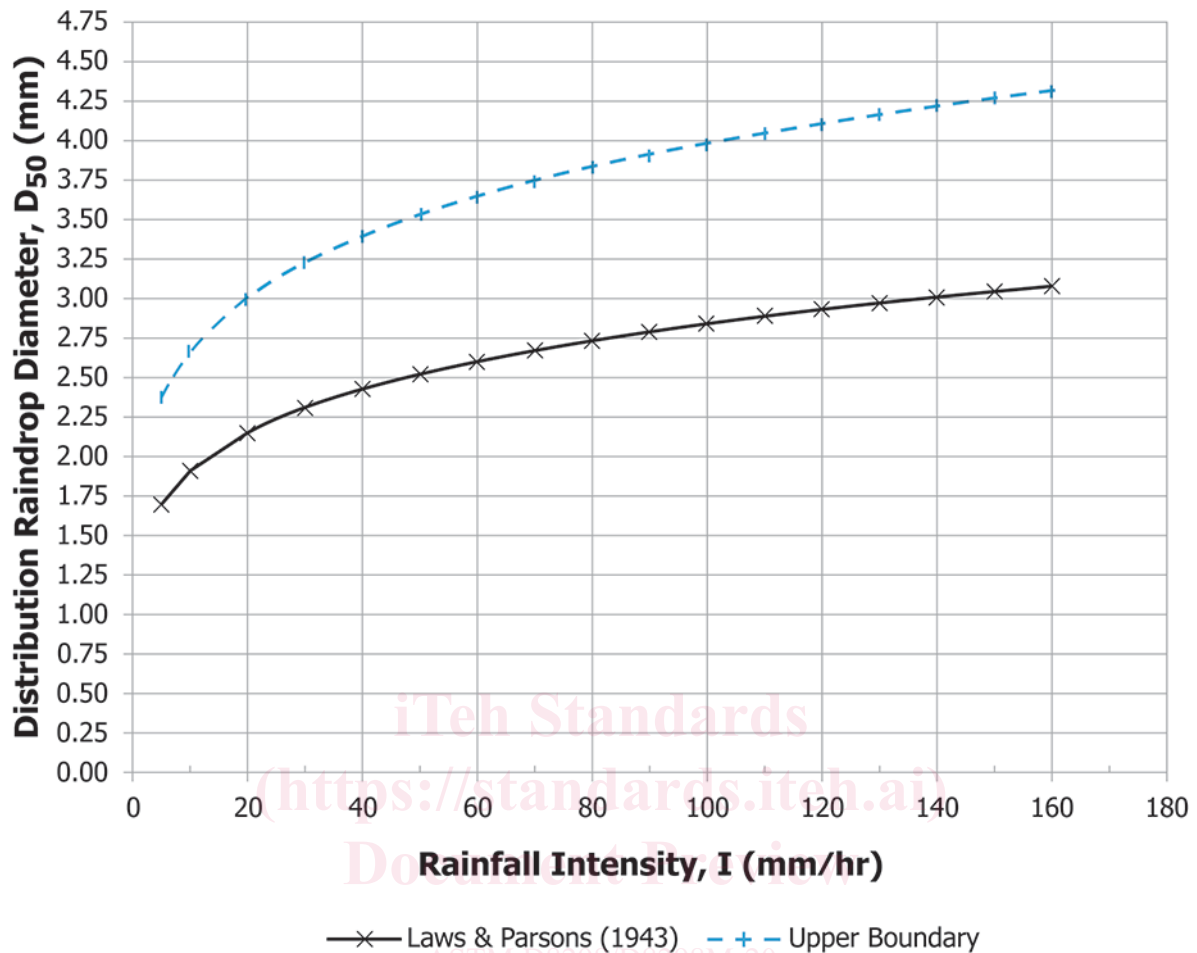
FIG. 1 Laws and Parsons (1943) Diameter-Intensity Plot
