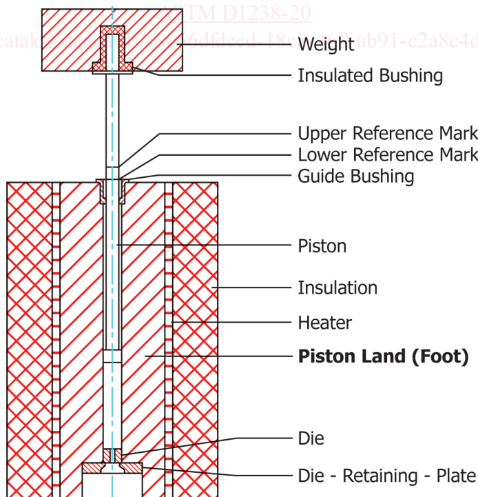
FIG. 1 General Arrangement of Extrusion Plastometer (See Section 56.)
