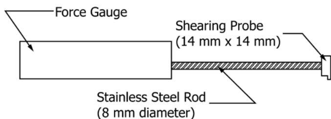
FIG. 1 Probe Design for the Detachment of Barnacles
