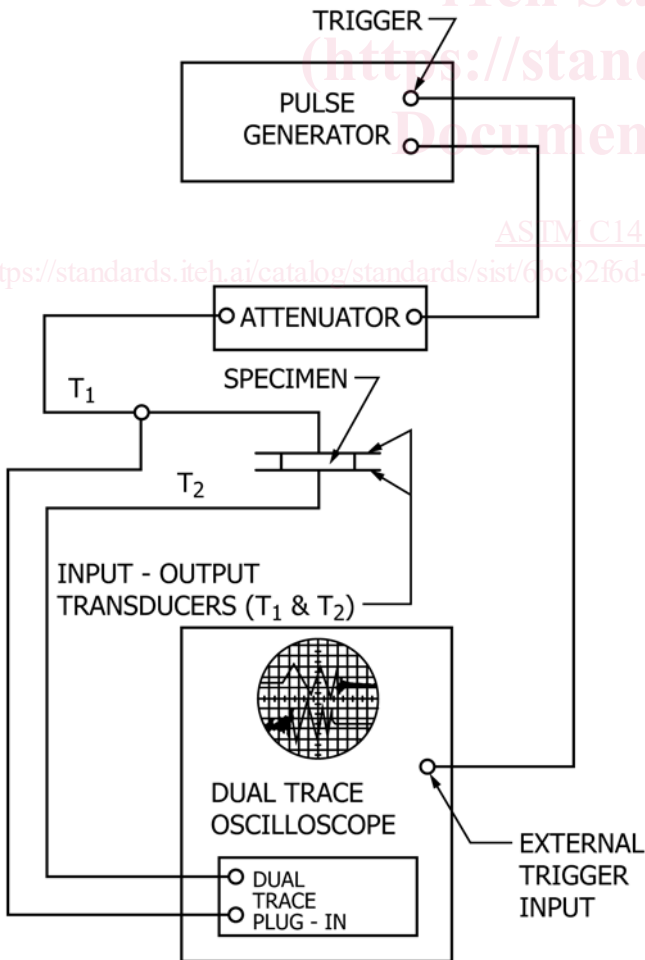
FIG. 1 Equipment Set-Up
