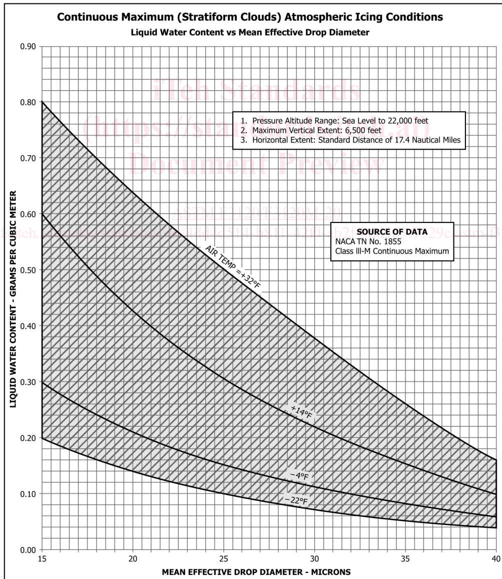
FIG. 1 Continuous Maximum (Stratiform Clouds) Icing Conditions – Liquid Water Content vs. LWC versus Mean Effective Drop Diameter
