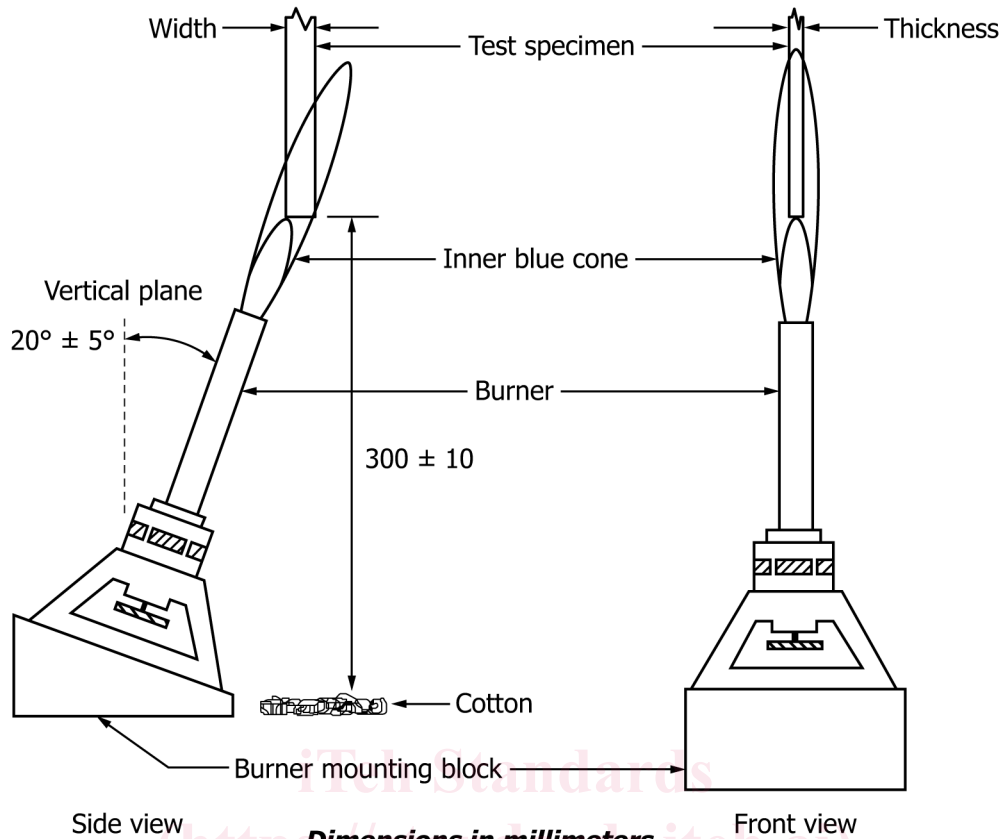
Dimensions in millimeters FIG. 2 Procedure A—Test of Bar Specimens
