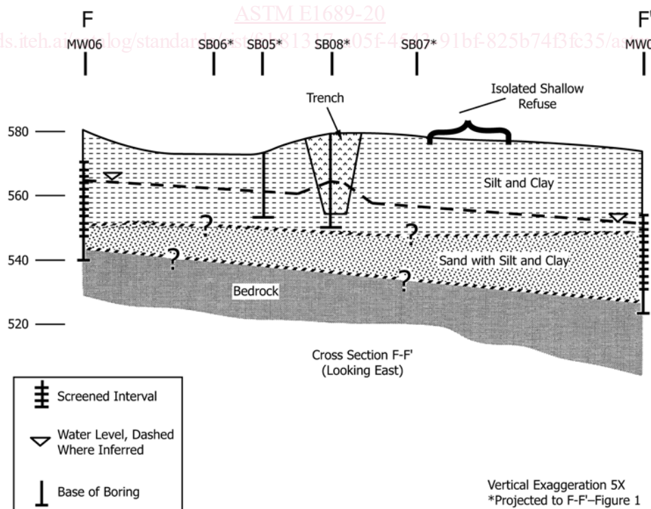
FIG. X1.2 Cross Section of Landfill Number 1
