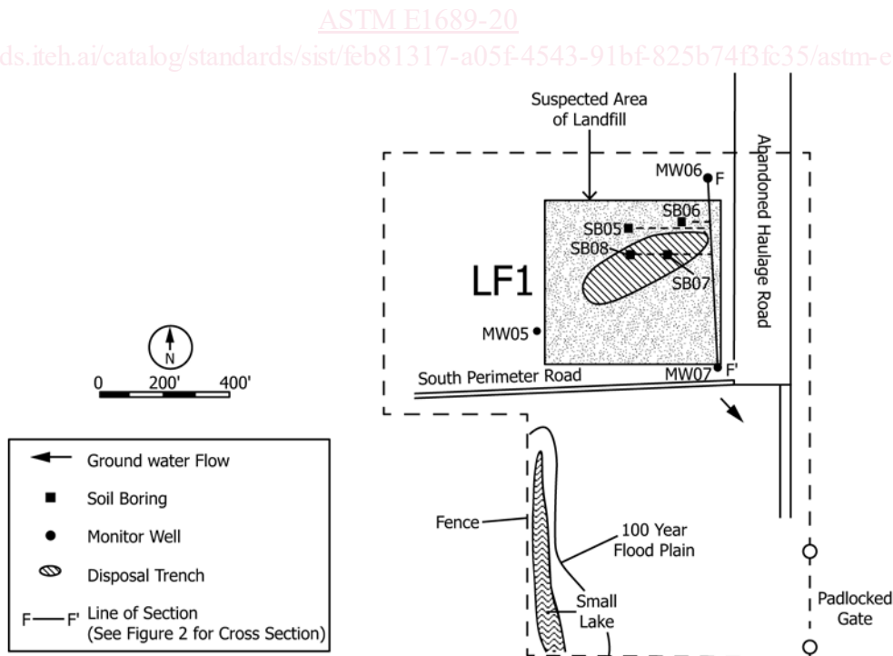
FIG. X1.1 Location Map for Landfill Number 1; Contours Showing the Potentiometric Surface from which Ground Water Flow Direction was Determined Could be Included in a Separate Figure to Avoid Clutter
