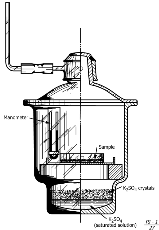
FIG. 1 Vacuum-Type Desiccator
