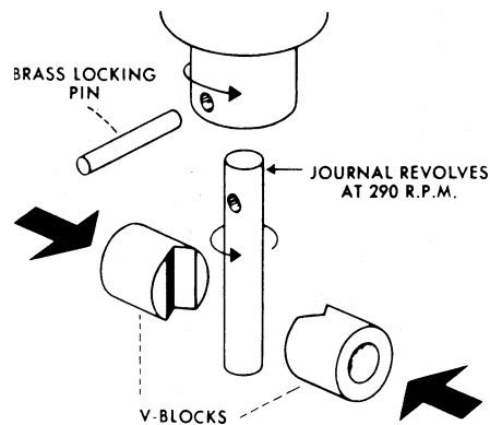
FIG. 2 Exploded View of Vee Blocks and Journal Arrangement, Failex Pin and Vee Block Test Machine
