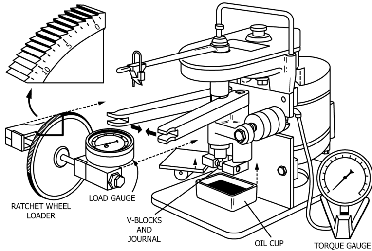
FIG. 1 Schematic Diagram of Failex Pin and Vee Block Test Machine
