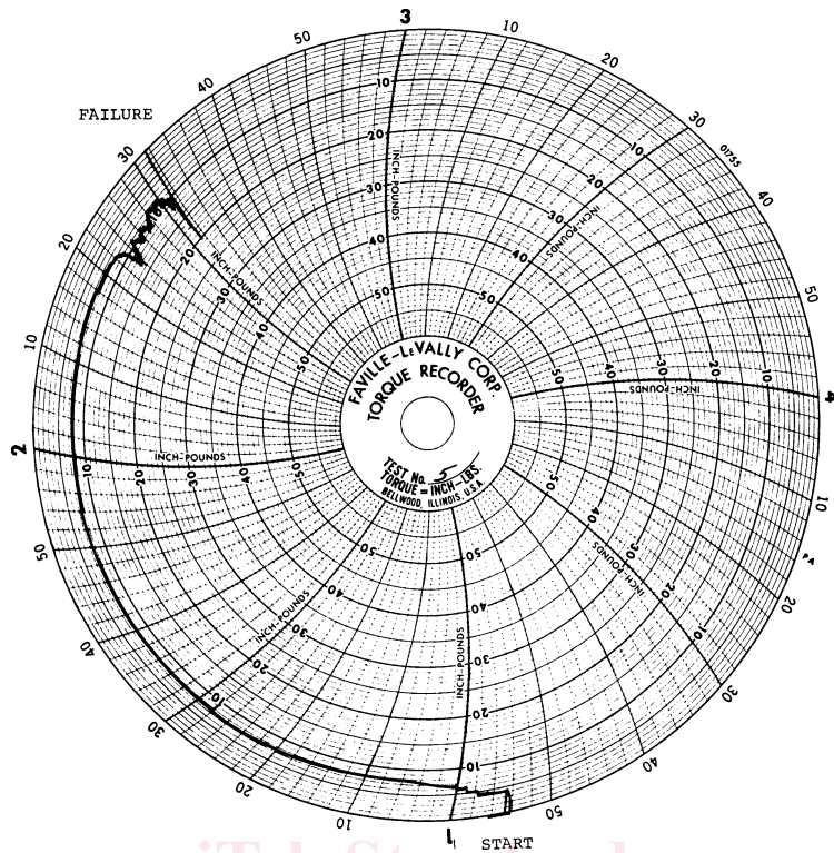
FIG. 5 Trace of Typical Torque Pattern for Procedure A, Using Falex Torque Recorder and Automatic Cutoff
