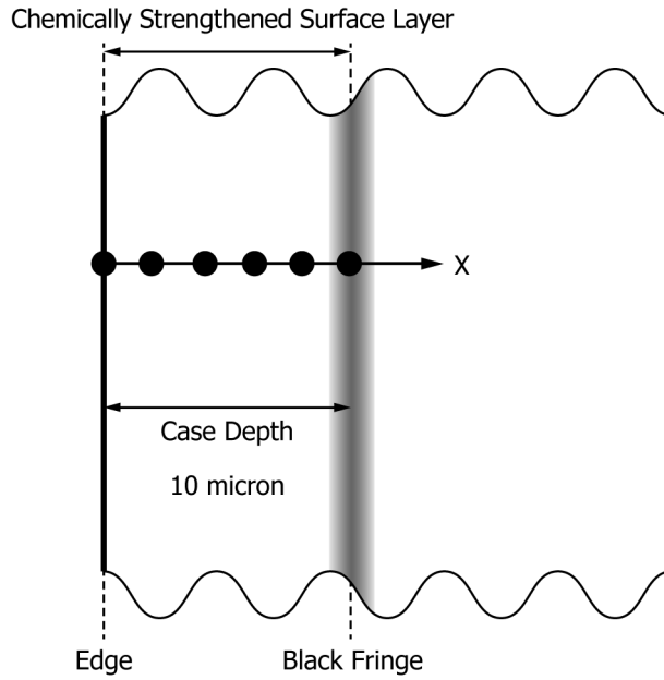
FIG. 23 (a) Case Depth and Birefringence Measurement Positions
