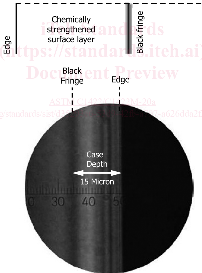
FIG. 23 (b) Photo from Polarizing Microscope Using Monochromatic Filter and Eyepiece Reticle to Measure Case Depth
