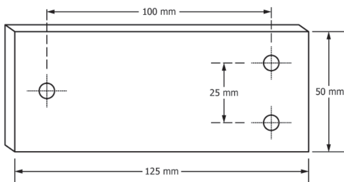
FIG. 4 Test Specimen
