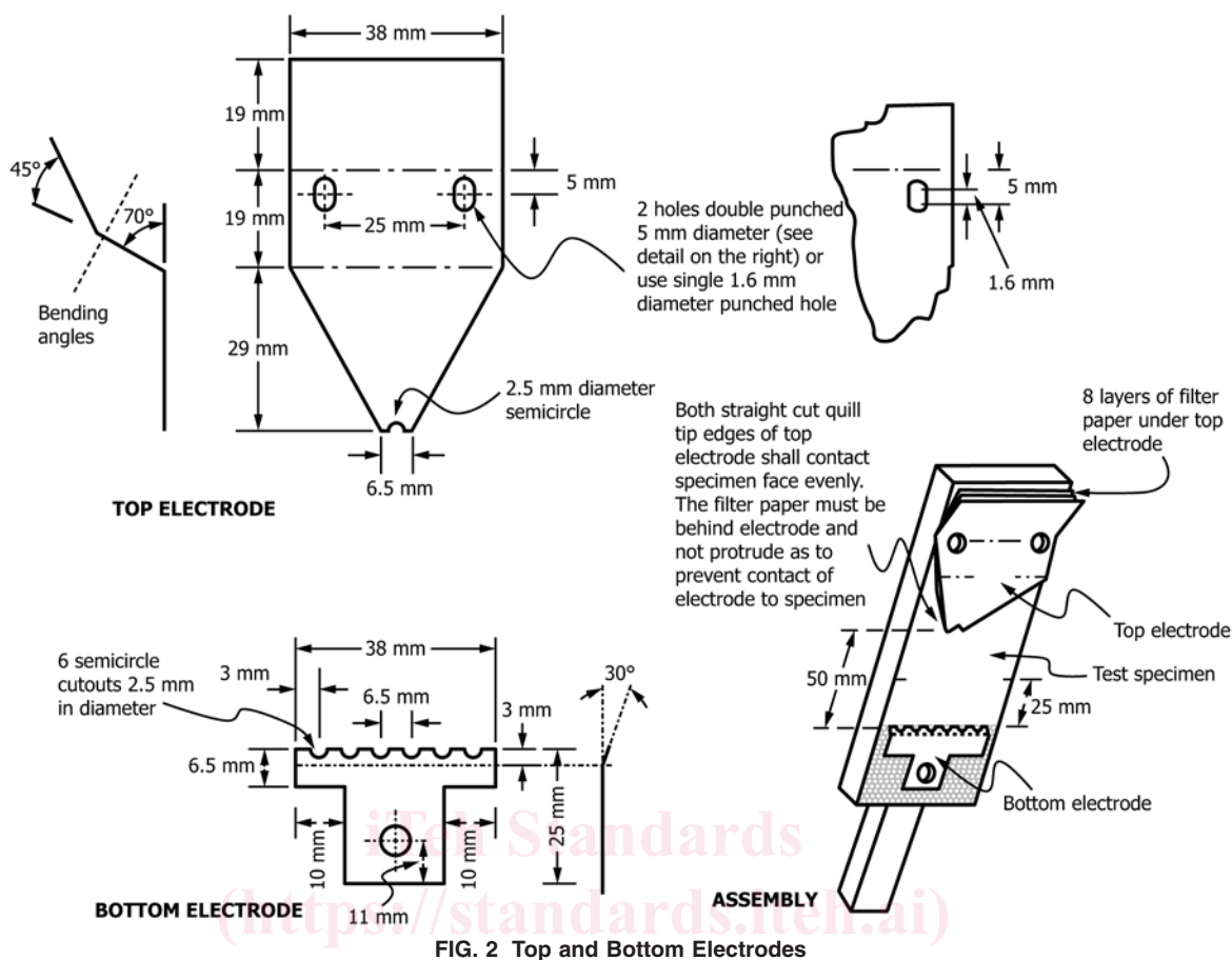
FIG. 2 Top and Bottom Electrodes
