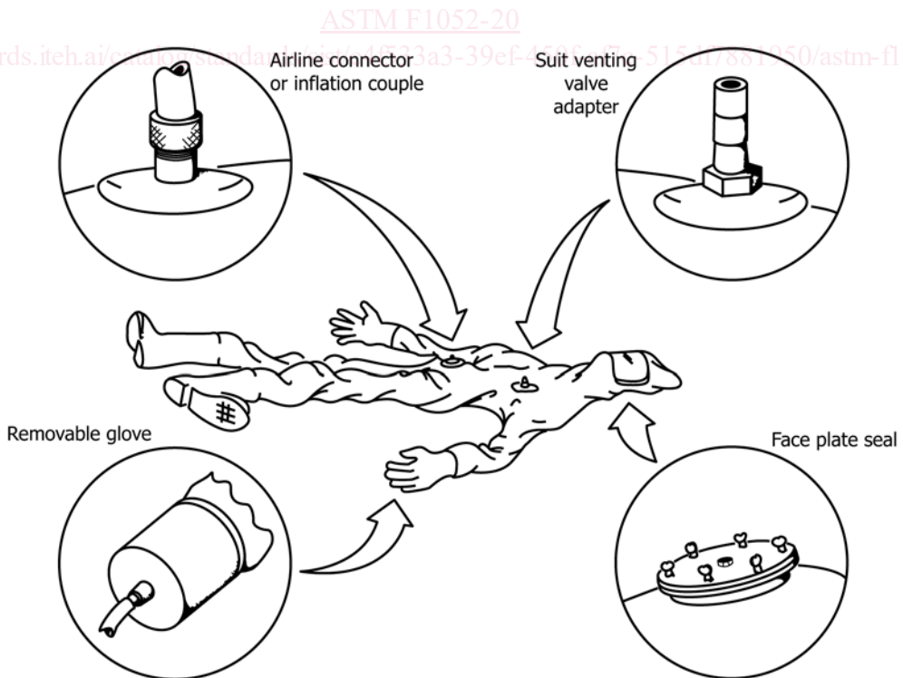
FIG. 1 Typical Examples of Suit Modification to Permit Inflation
