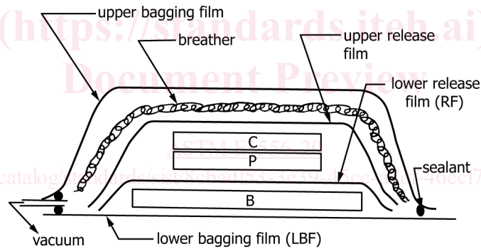
FIG. 2 Layout Scheme for Tensile Lap Shear Panel
